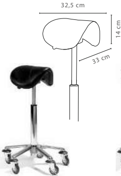
02003 02 / Saddle
