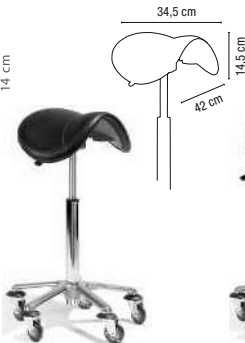
02004 03 / Saddle XL
